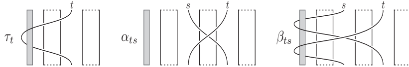
Figure 1: Braid pictures for type B new generators.
