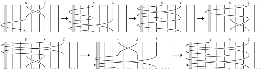
Figure 2: Type B braid isotopies. Figure 2: Isotopies de tresses de type B.
