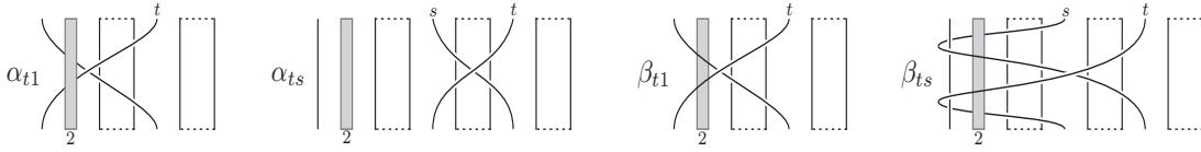
Figure 3: Braid pictures for type D new generators.
