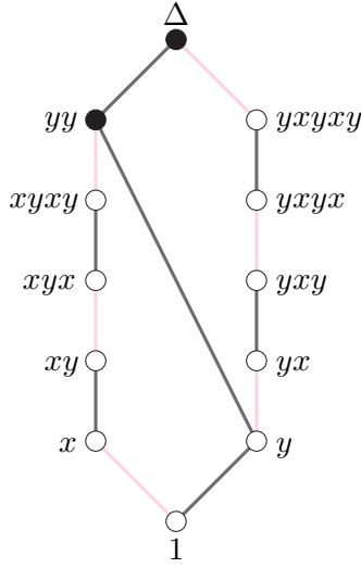
Figure 2. The lattice (S_{\bullet}, \vee, \wedge) of simples in M_{\bullet} .
